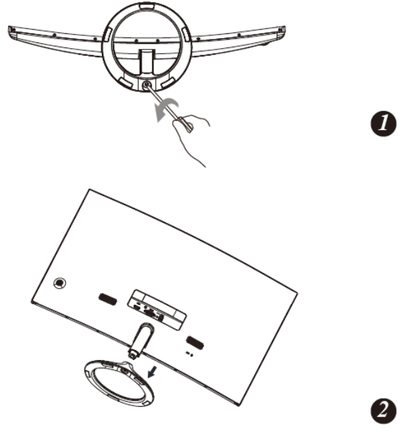
Figure.1. Installing and Removing the Base
