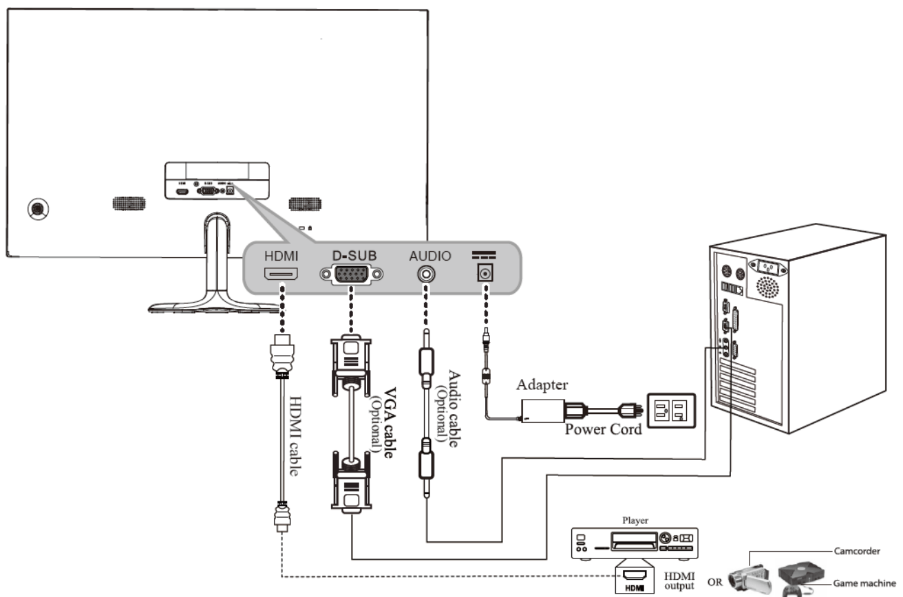
Figure.2. Connecting to a PC
